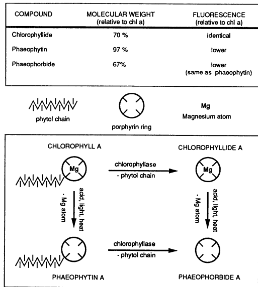
FIG. 1. The relative properties of chlorophyll a and its degradation products, the primary components of the molecules, and a schematic of the degradation of chlorophyll into its degraded forms. As a result of the similarities in fluorescence characteristics, chlorophyll and chlorophyllide cannot be distinguished fluorometrically, nor can phaeophytin and phaeophorbide. The convention among users of the gut fluorescence technique is to refer to phaeophytin and phaeophorbide collectively as phaeopigments.
