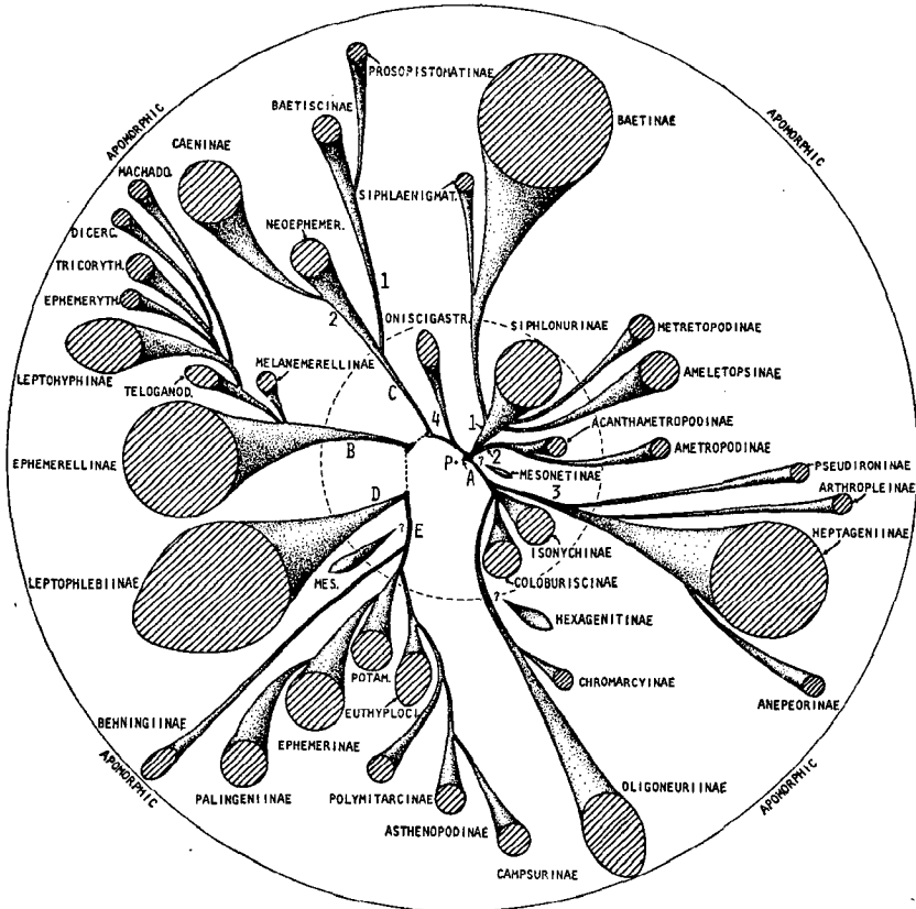
FIG. 1. "End-view" diagram of the probable phylogeny of the subfamilies of Ephemeroptera. The Permian families are not indicated. The center (P) is the point of ancestral plesiomorphy. Increasing apomorphy is indicated by distance from the center. The extant diversity of the subfamily is indicated by the area of the end of the lineage. Fossil subfamilies end as points. The interior dotted circle encloses the evolutionary grade limits of the Siphonuridae. (The position of the Ameletopsinae on this diagram is not a proposal for family category.) See discussion for assumptions on times of branching and family classifications. For most abbreviated names add "inae" only; others abbreviated as follows: Machado = Machadorythinae; Dicerco = Dicercomyzinae; Potam = Potamanthinae; and Mes = Mesepheemerinae.
