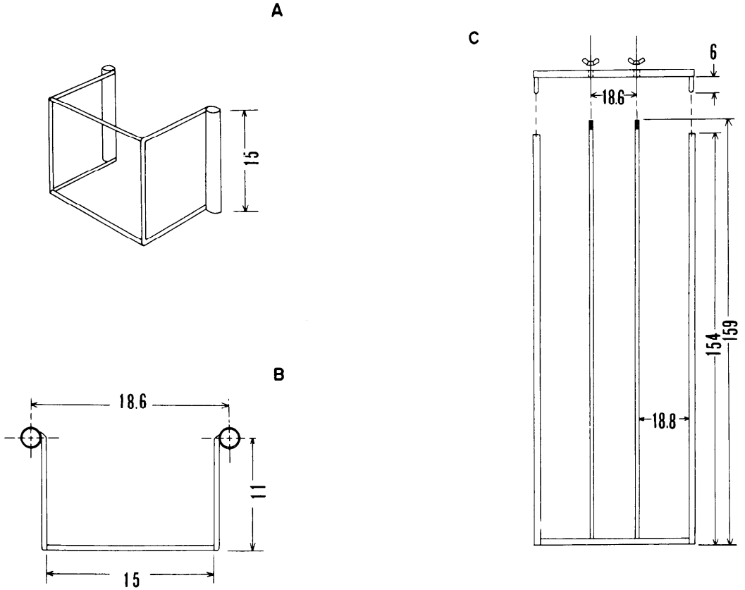
Fig. 1. A, B—Brass rod drift net frame with steel conduit attachment tubes; C—net-stack frame with center rods to receive conduit tubes of net frames. (Numbers = centimeters.)
