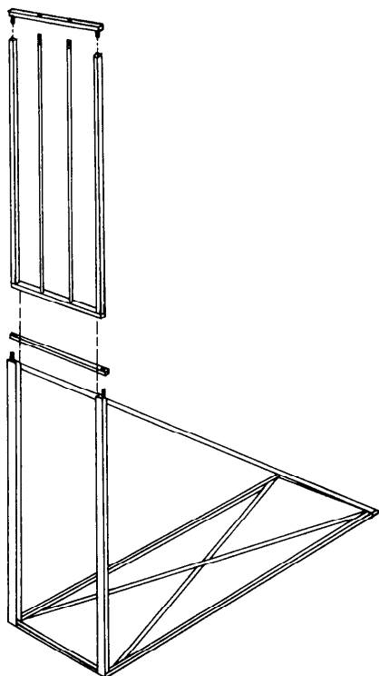
Fig. 2. Alignment of net-stack frame and channels at anterior face of fixed river frame.
