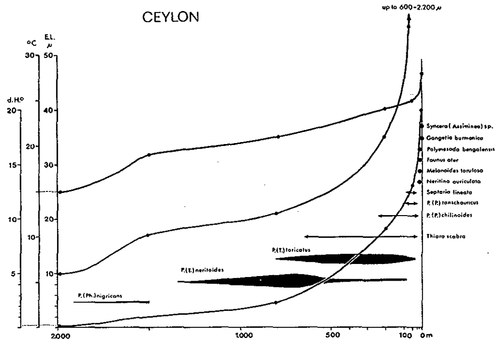
Fig. 4. Diagram showing temperature, hardness degree and electrolytic conductivity of the running waters correlated with the longitudinal distribution of the freshwater gastropods and bivalves between headwaters and the mouth of mountain streams of Southern Sri Lanka (Temperature in °Celsius; Total hardness in °dH (German hardness degree); Electrolytic conductivity ( El_{20} ) in \mu Siemens (at 20° Celsius) (After STARMÜHLNER, 1979b).
